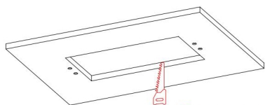
③ Cut-out: 251*128MM
